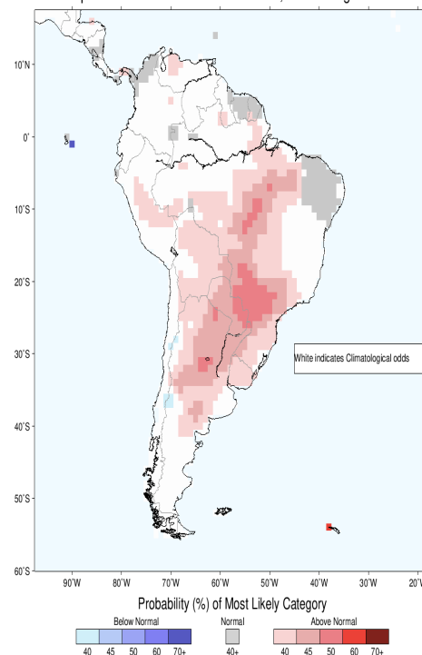
IRI Multi-Model Probability Forecast for Temperature for September–October–November 2020, Issued August 2020
