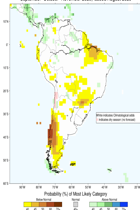
IRI Multi-Model Probability Forecast for Precipitation for September–October–November 2020, Issued August 2020
