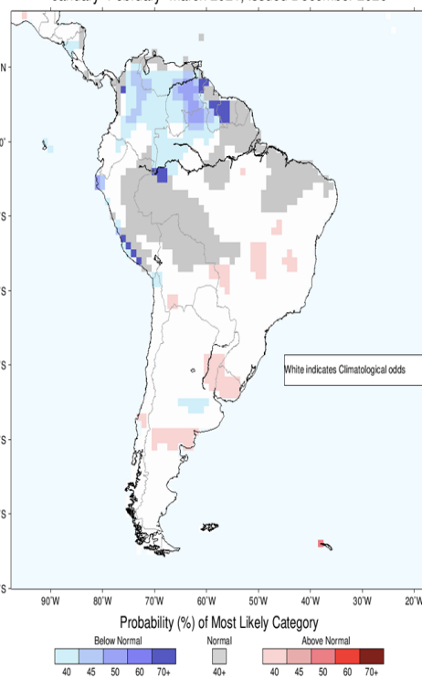
IRI Multi-Model Probability Forecast for Temperature for January-February-March 2021, Issued December 2020
