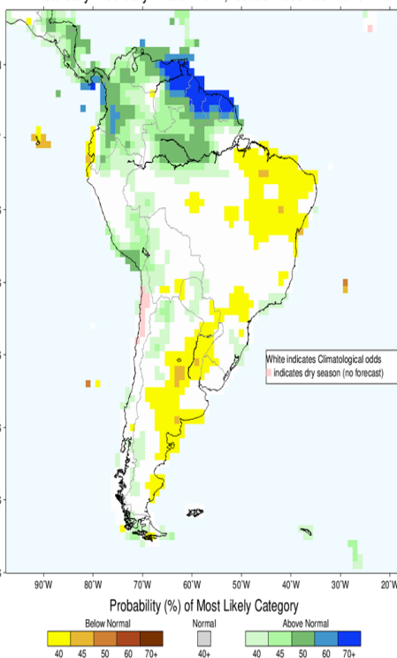
IRI Multi-Model Probability Forecast for Precipitation for January-February-March 2021, Issued December 2020
