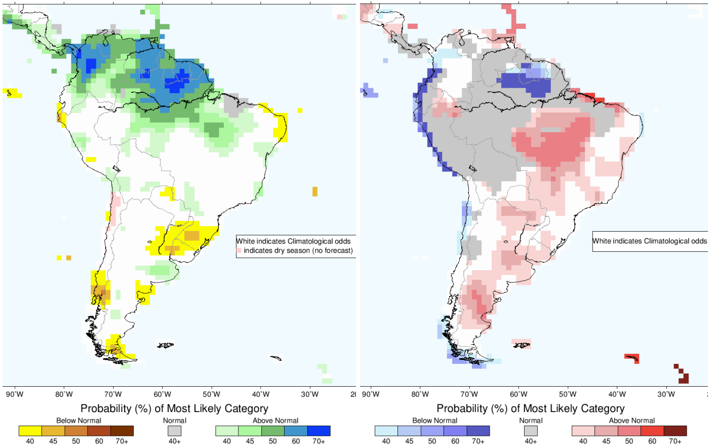
IRI Multi-Model Probability Forecast for Precipitation for January-February-March 2022, Issued December 2021
